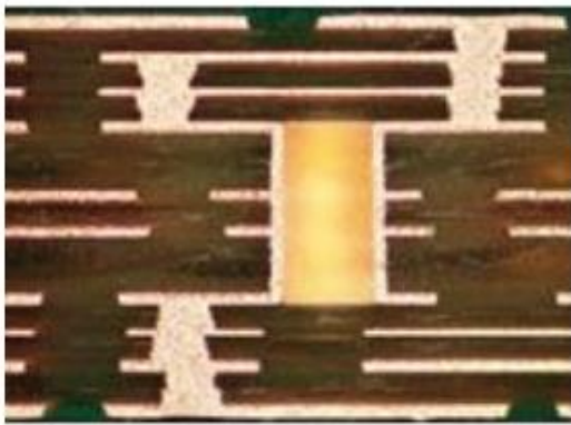
3阶HDI
