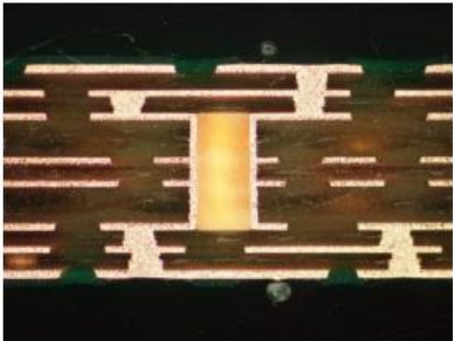
2阶HDI
